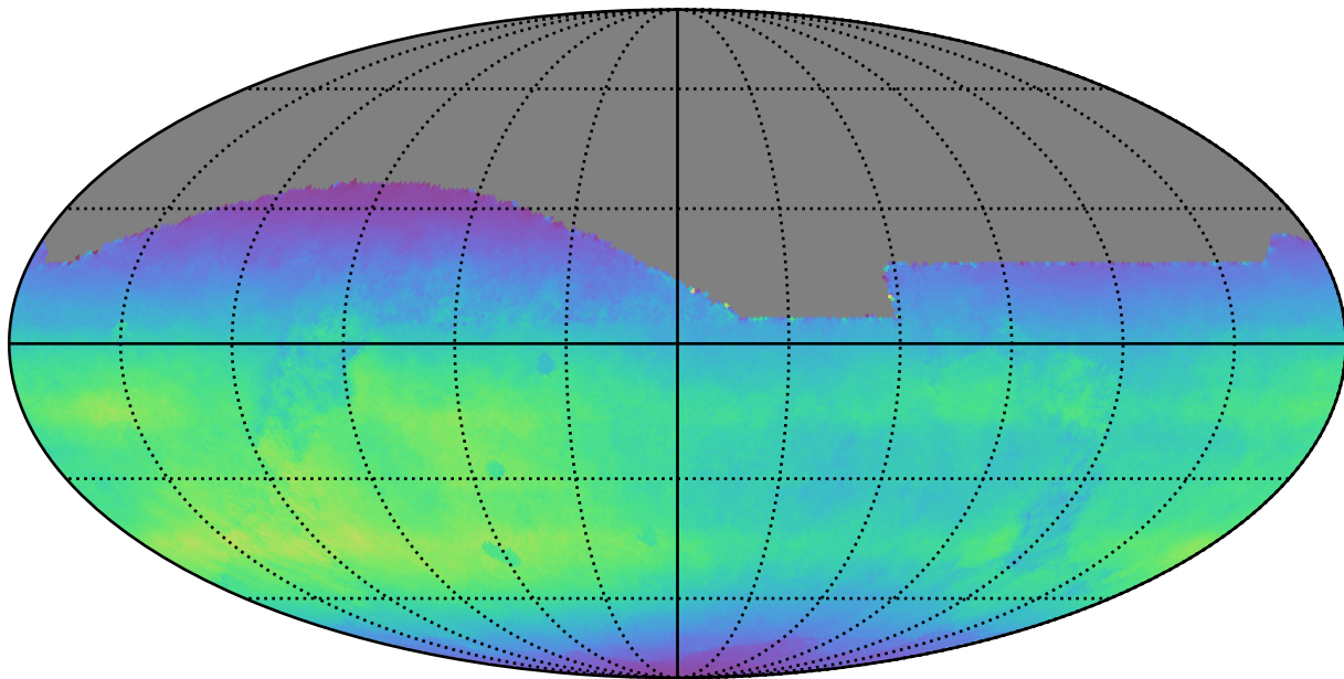
ddf_acor_sf15_lsf20_lsr10_v3.4_10yrs All sky all bands: Normalized Teff
