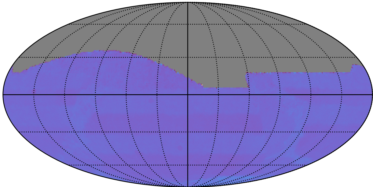
ddf_acor_sf15_lsf20_lsr10_v3.4_10yrs All sky: Normalized Proper Motion Uncert @ 20.5
