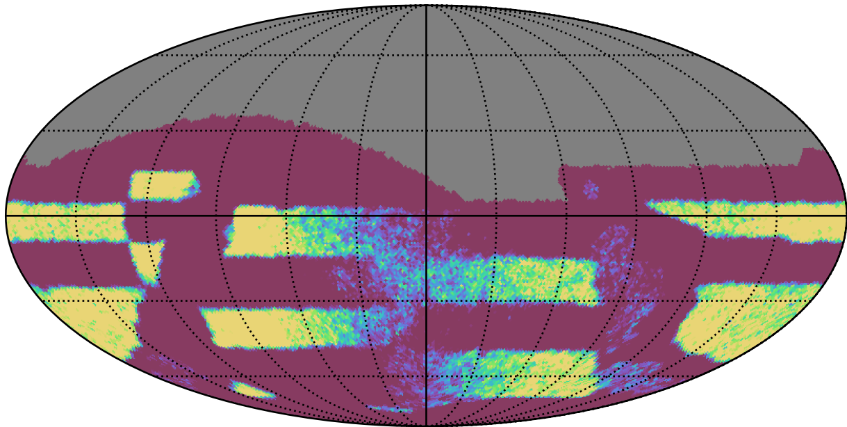
ddf_acor_sf15_lsf20_lsr10_v3.4_10yrs Yr 3-4 all bands: NVisits
