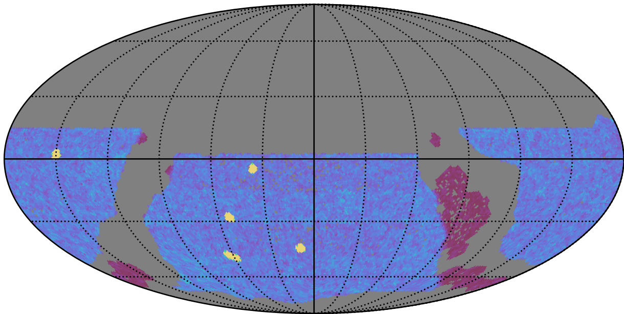
ddf_acor_sf15_lsf20_lsr10_v3.4_10yrs WFD y band: NVisits
