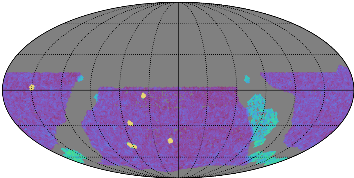
ddf_acor_sf15_lsf20_lsr10_v3.4_10yrs WFD g band: NVisits
