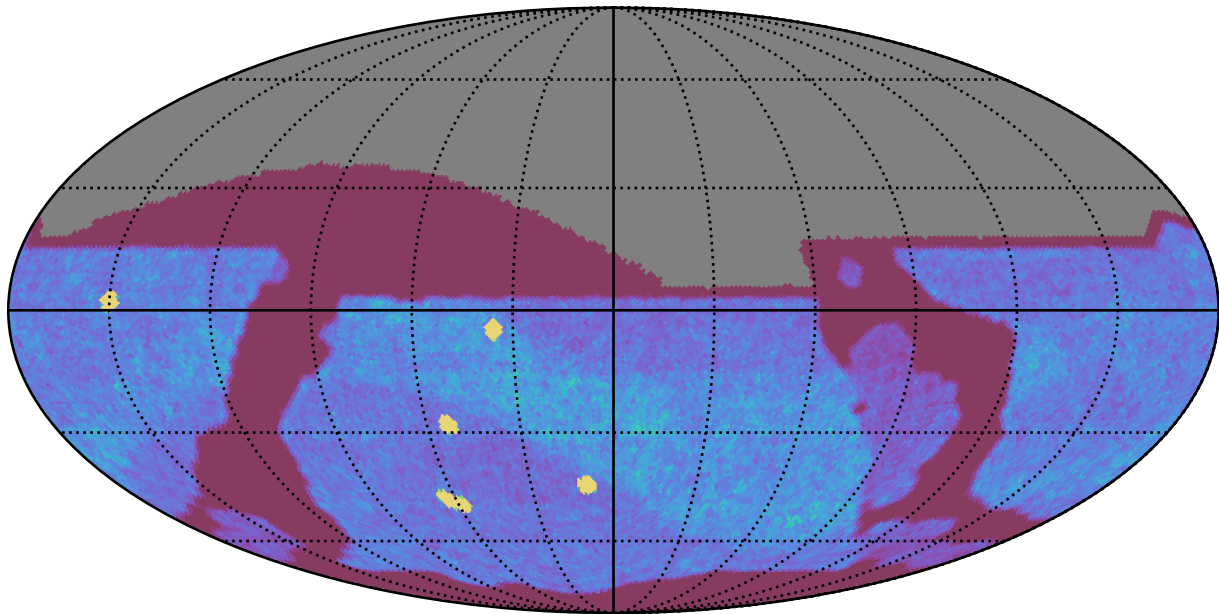
ddf_acor_sf15_lsf20_lsr10_v3.4_10yrs All sky z band: NVisits
