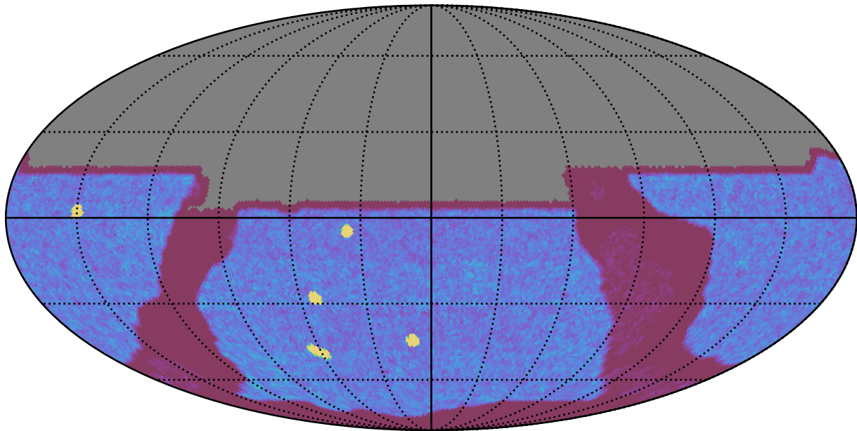
ddf_acor_sf15_lsf20_lsr10_v3.4_10yrs All sky y band: NVisits
