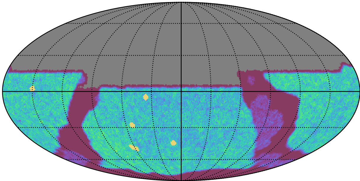
ddf_acor_sf15_lsf20_lsr10_v3.4_10yrs All sky u band: NVisits
