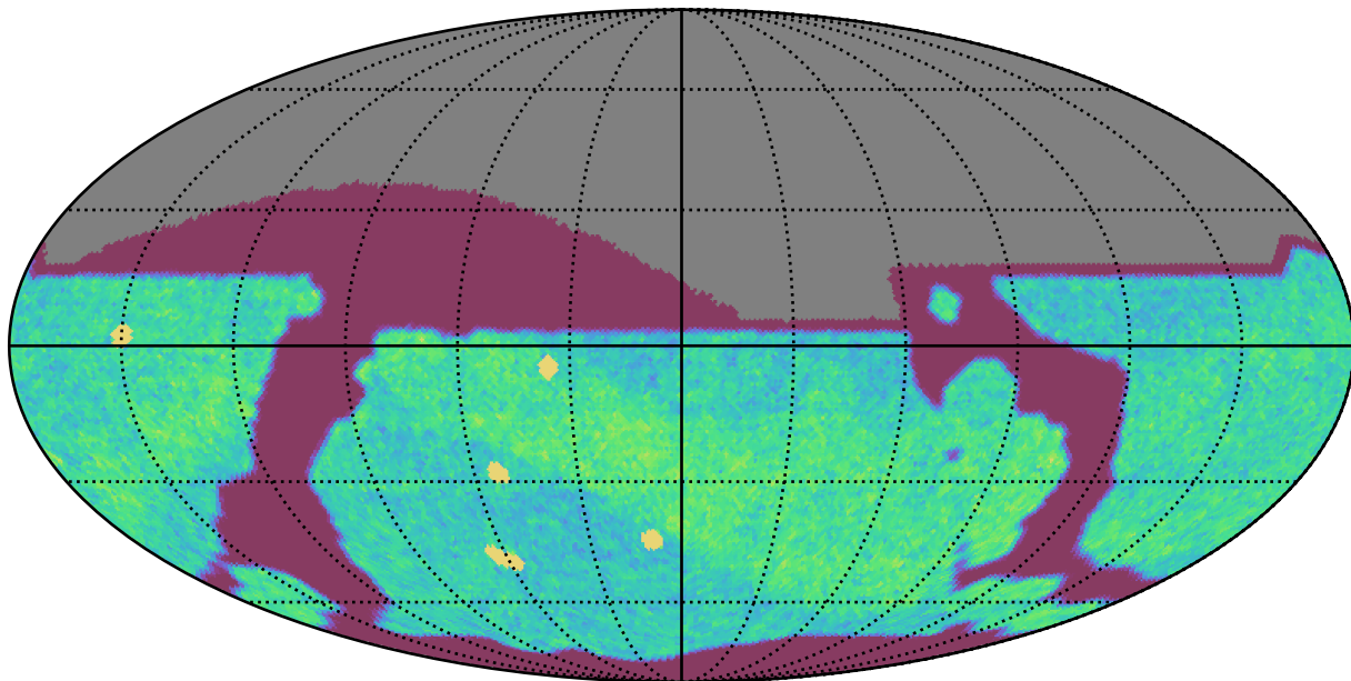
ddf_acor_sf15_lsf20_lsr10_v3.4_10yrs All sky i band: NVisits
