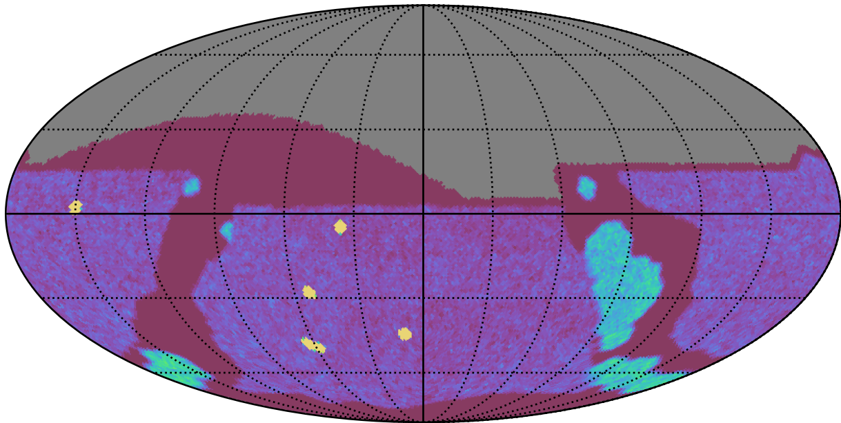
ddf_acor_sf15_lsf20_lsr10_v3.4_10yrs All sky g band: NVisits
