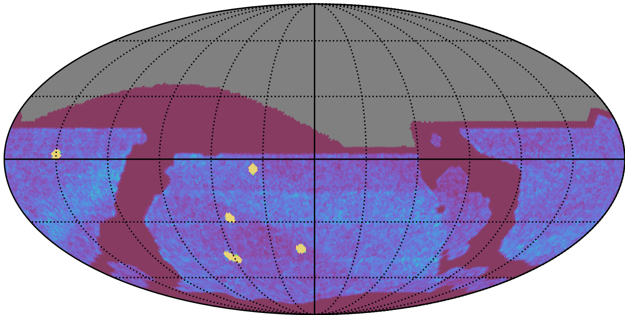
ddf_acor_sf15_lsf20_lsr10_v3.4_10yrs All sky all bands: NVisits
