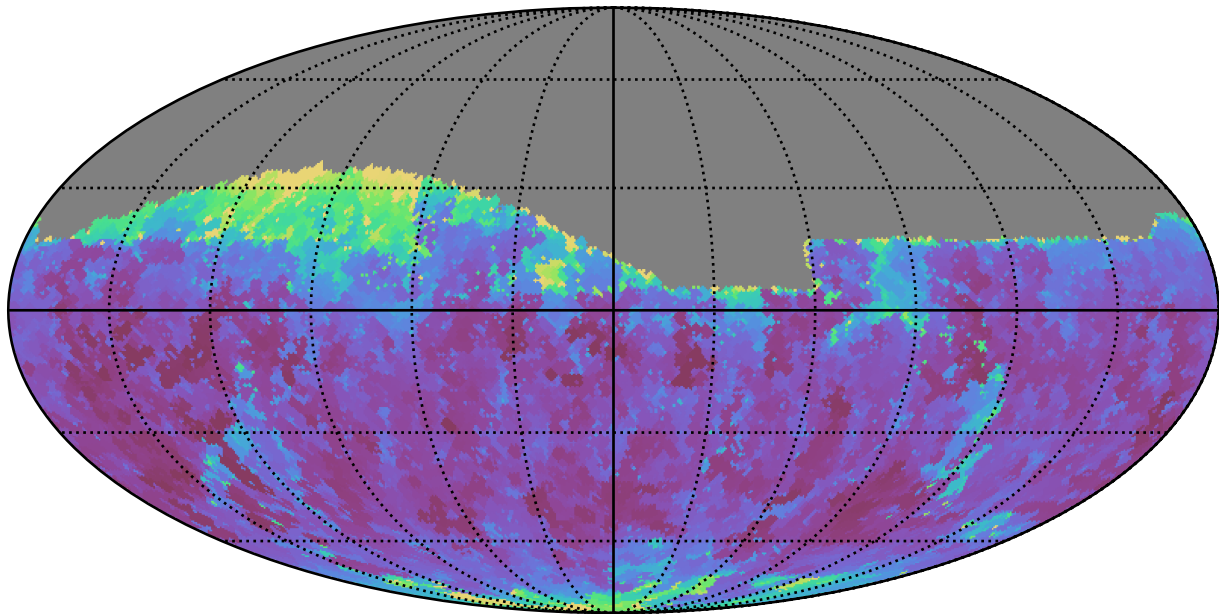
ddf_acor_sf15_lsf20_lsr10_v3.4_10yrs Yr 1 z band: Min seeingEff
