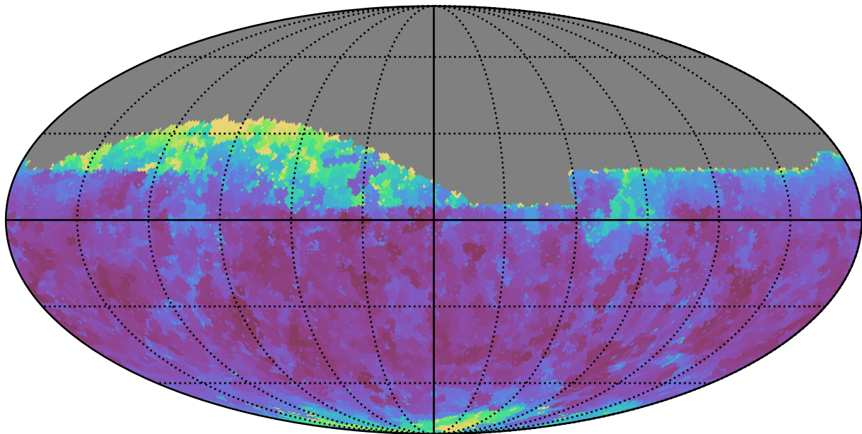
ddf_acor_sf15_lsf20_lsr10_v3.4_10yrs Yr 1 i band: Min seeingEff
