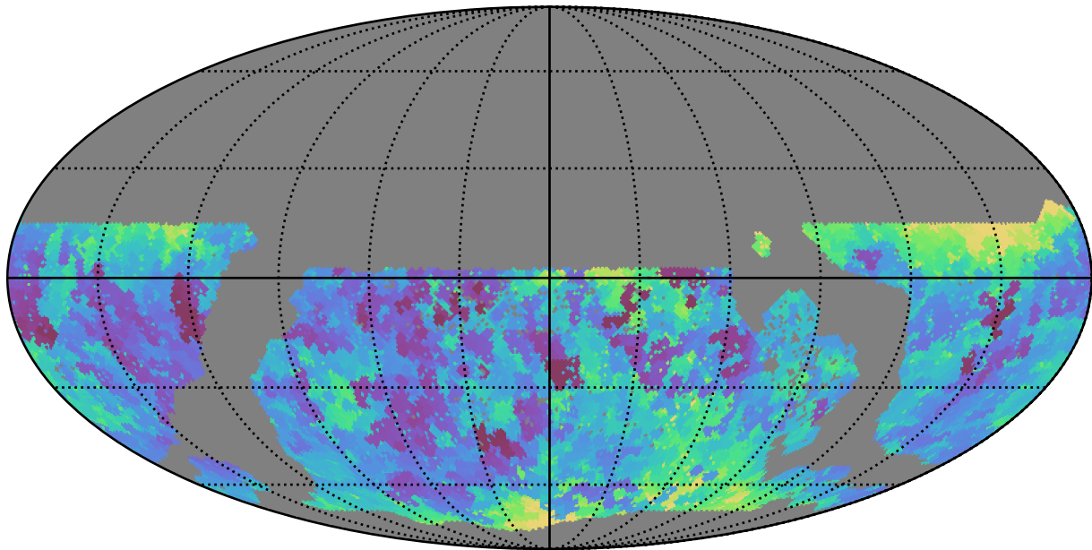
ddf_acor_sf15_lsf20_lsr10_v3.4_10yrs WFD g band: Min seeingEff
