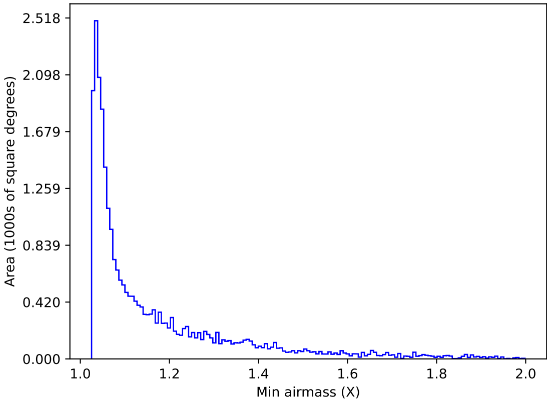
ddf_acor_sf15_lsf20_lsr10_v3.4_10yrs Yr 1 z band: Min airmass
