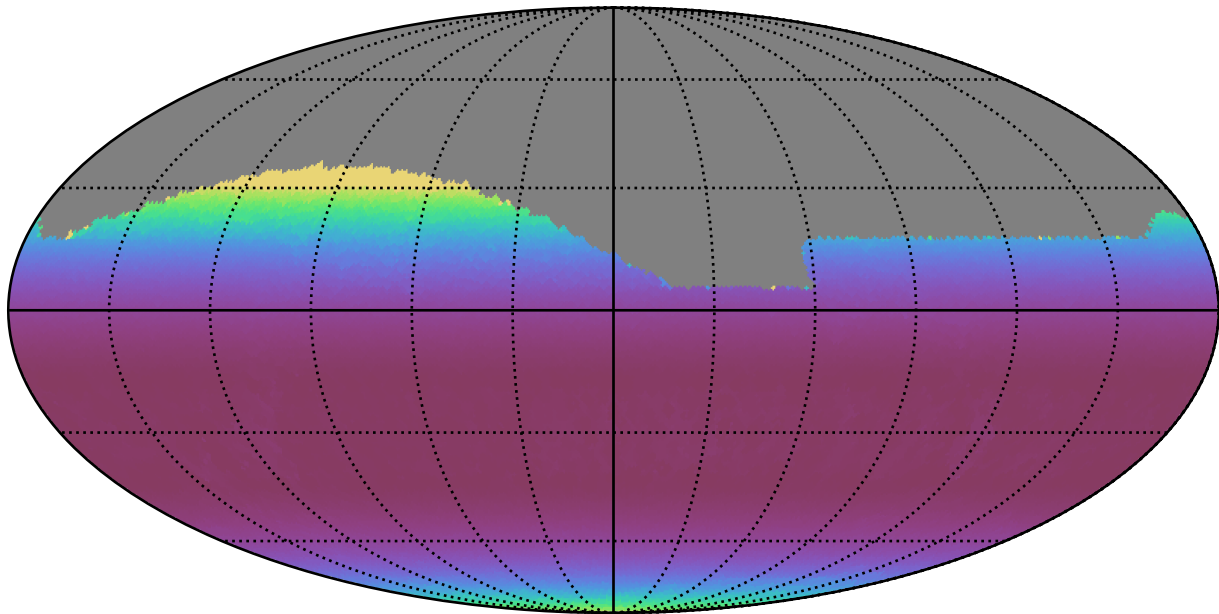
ddf_acor_sf15_lsf20_lsr10_v3.4_10yrs Yr 1 all bands: Min airmass
