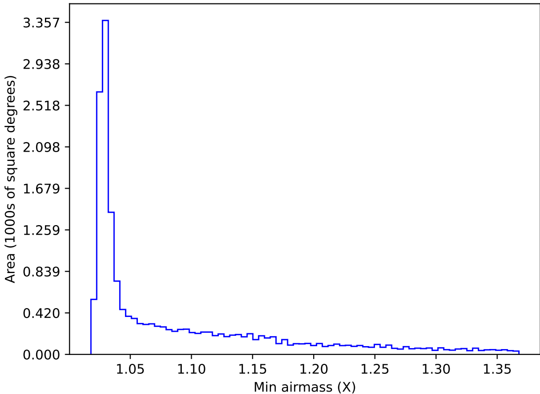
ddf_acor_sf15_lsf20_lsr10_v3.4_10yrs WFD z band: Min airmass
