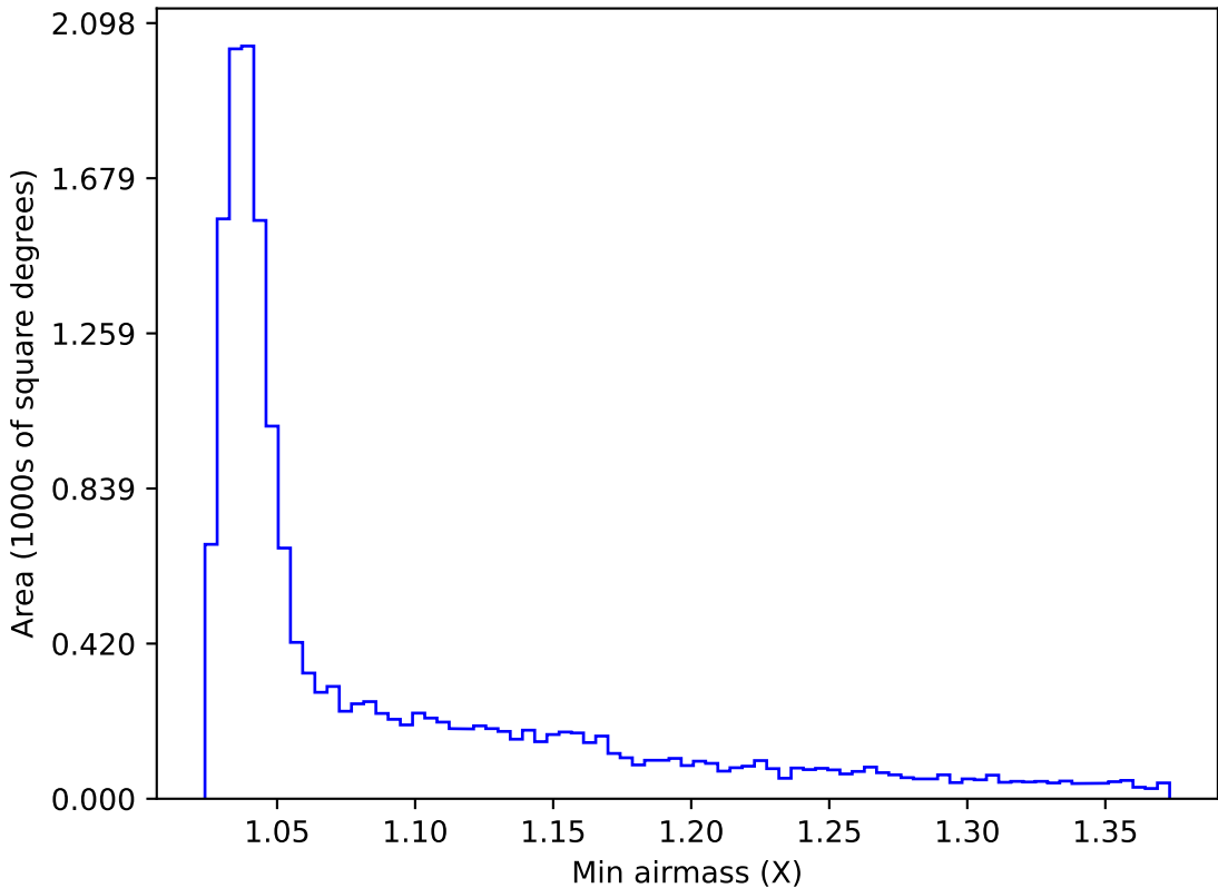
ddf_acor_sf15_lsf20_lsr10_v3.4_10yrs WFD u band: Min airmass
