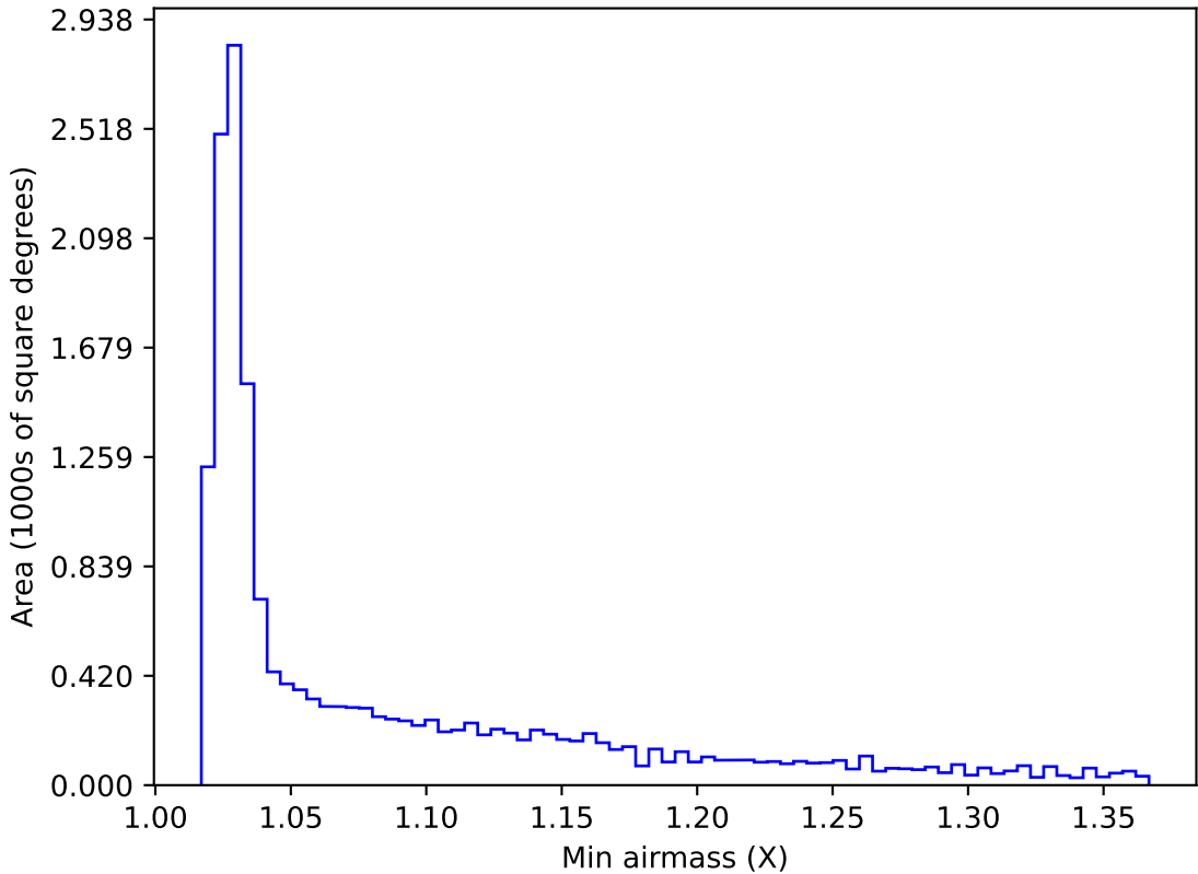
ddf_acor_sf15_lsf20_lsr10_v3.4_10yrs WFD r band: Min airmass
