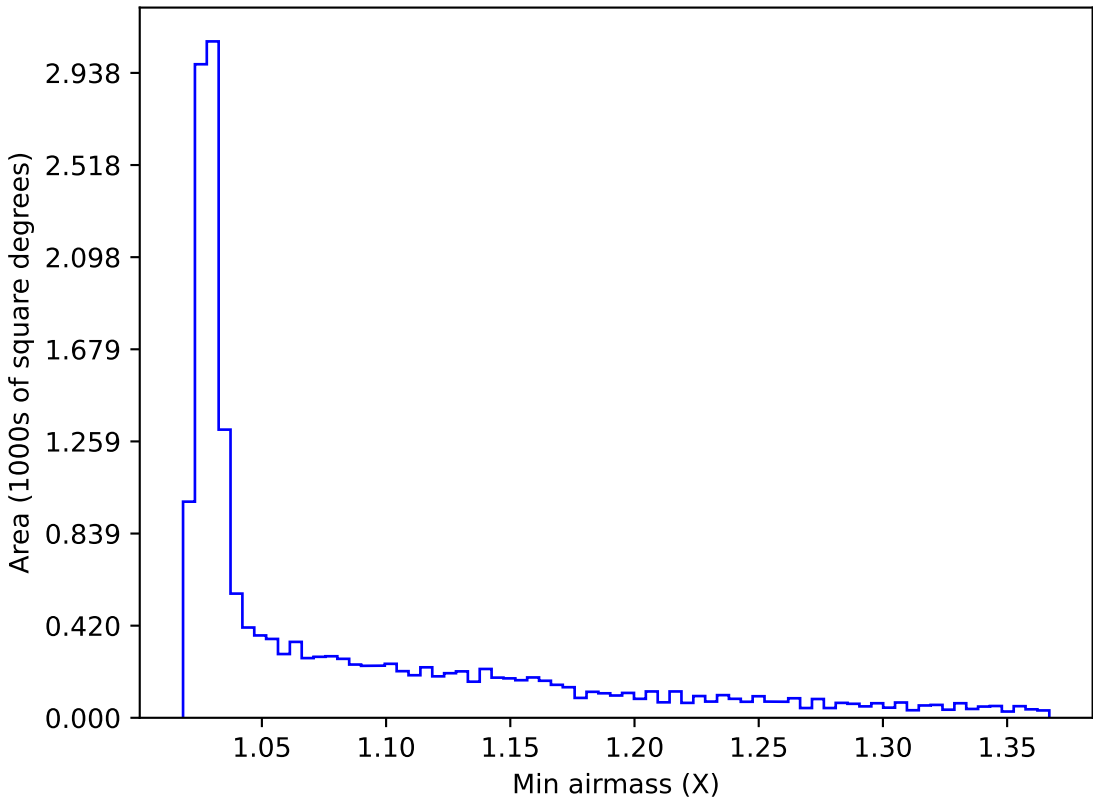
ddf_acor_sf15_lsf20_lsr10_v3.4_10yrs WFD i band: Min airmass
