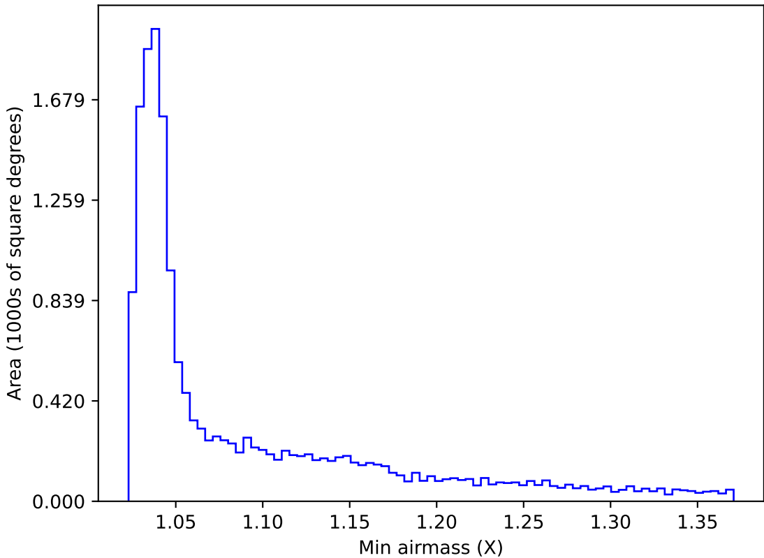
ddf_acor_sf15_lsf20_lsr10_v3.4_10yrs WFD g band: Min airmass
