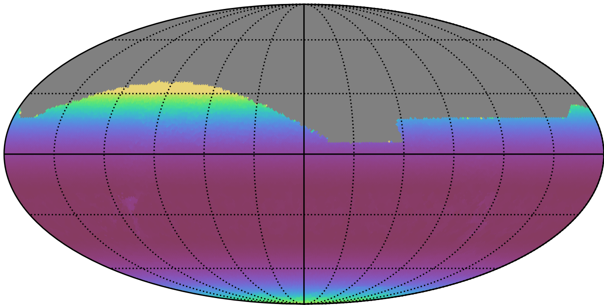
ddf_acor_sf15_lsf20_lsr10_v3.4_10yrs All sky z band: Min airmass
