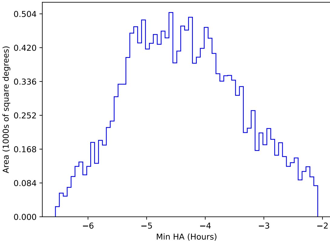
ddf_acor_sf15_lsf20_lsr10_v3.4_10yrs WFD z band: Min HA
