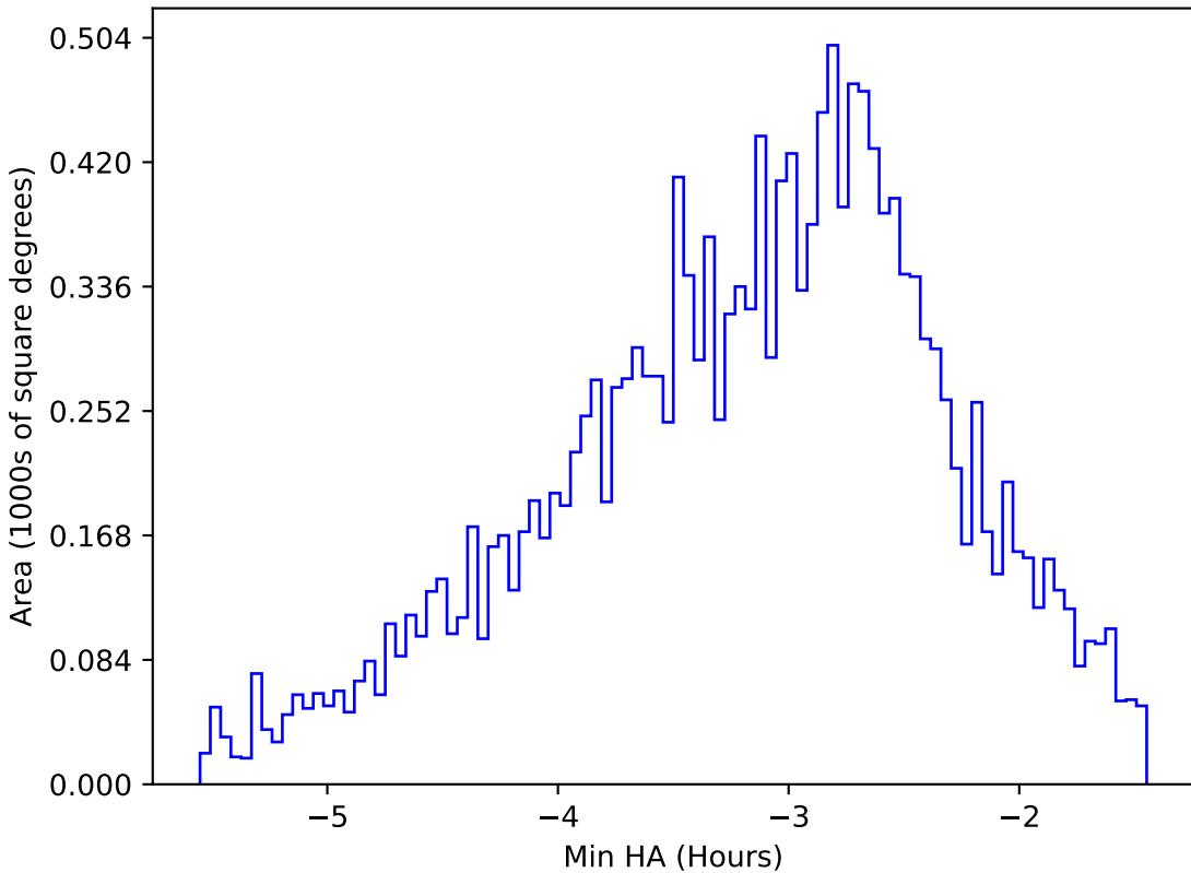
ddf_acor_sf15_lsf20_lsr10_v3.4_10yrs WFD u band: Min HA
