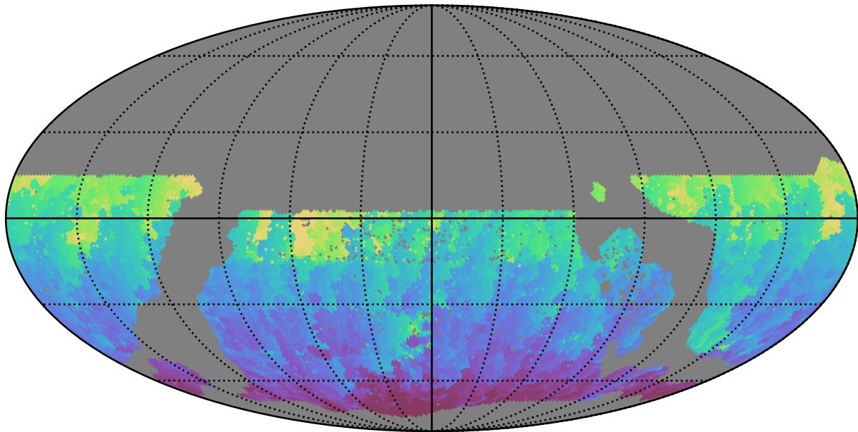
ddf_acor_sf15_lsf20_lsr10_v3.4_10yrs WFD g band: Min HA
