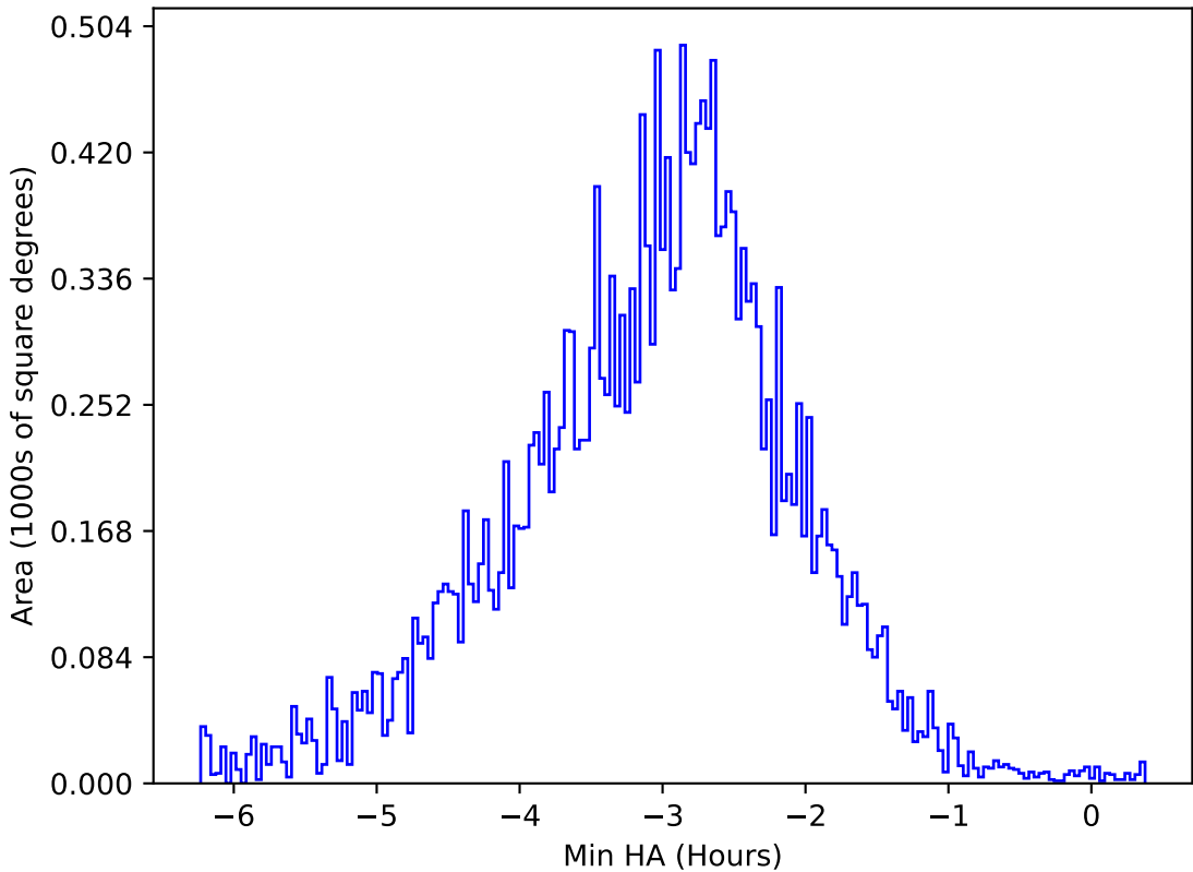
ddf_acor_sf15_ls20_lsr10_v3.4_10yrs All sky u band: Min HA
