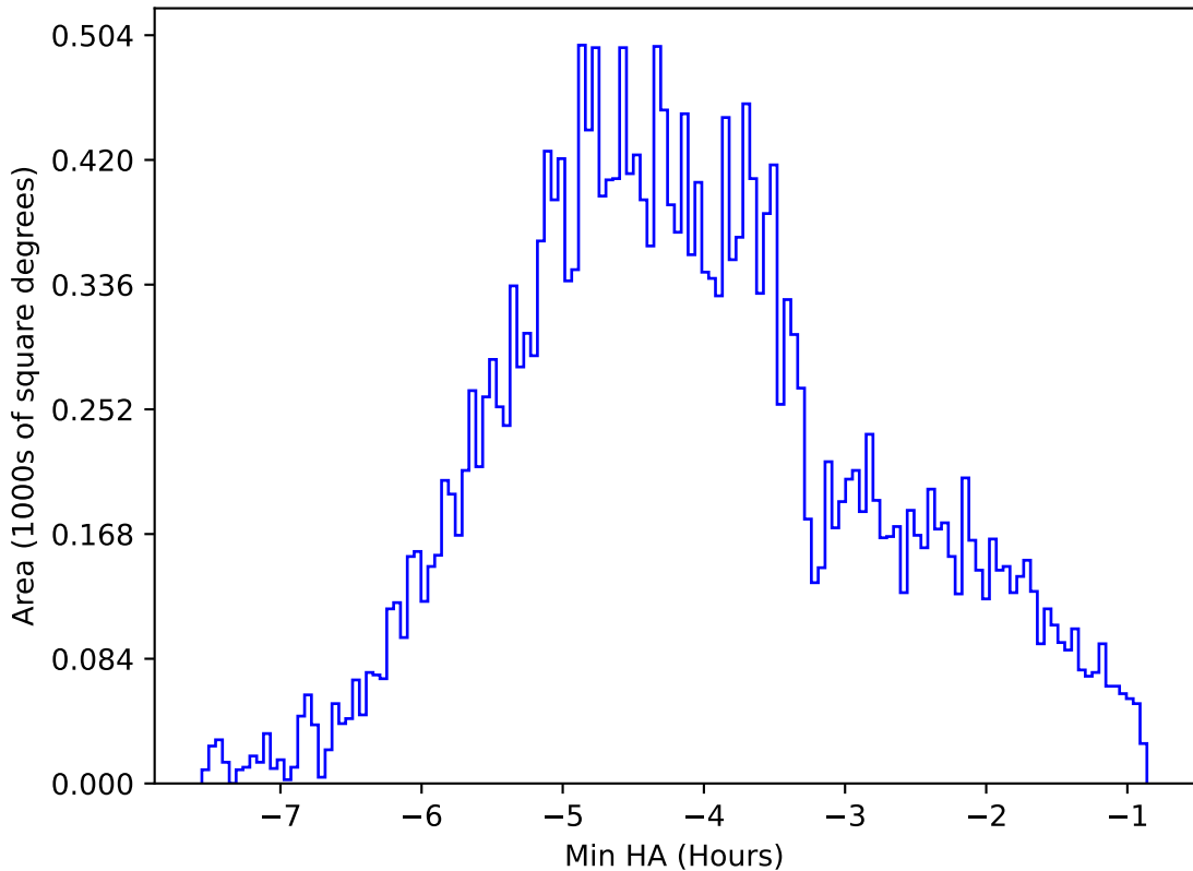
ddf_acor_sf15_lsf20_lsr10_v3.4_10yrs All sky i band: Min HA
