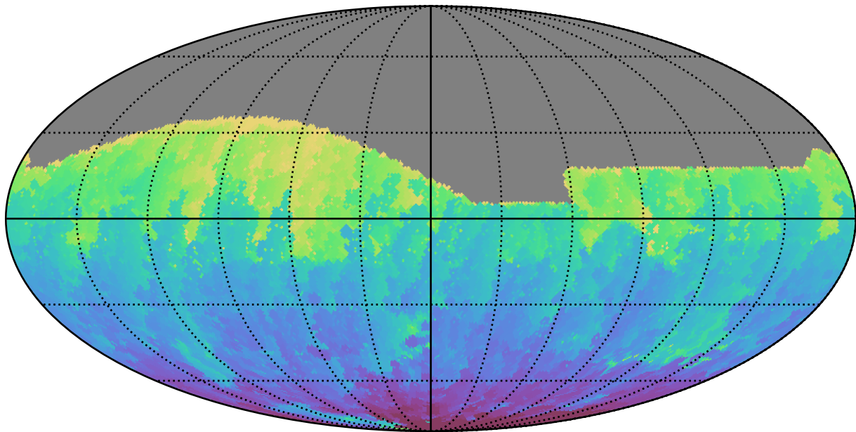
ddf_acor_sf15_lsf20_lsr10_v3.4_10yrs All sky g band: Min HA
