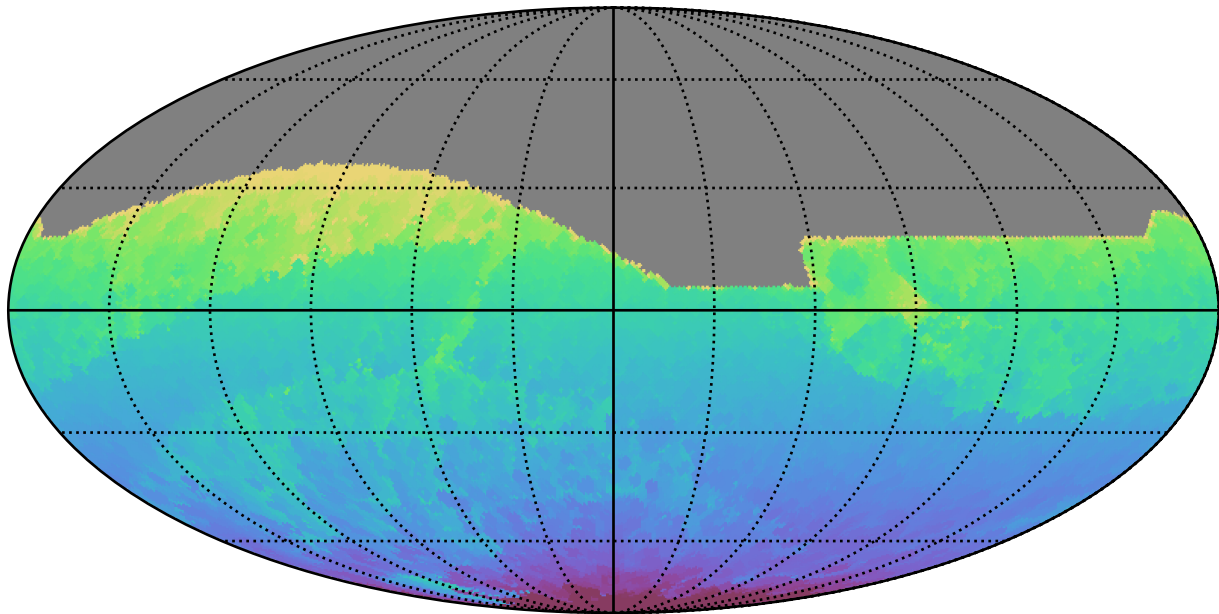
ddf_acor_sf15_lsf20_lsr10_v3.4_10yrs All sky all bands: Min HA
