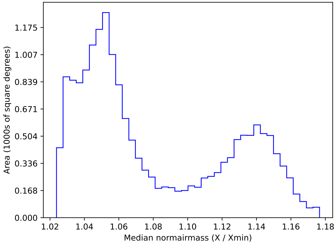
ddf_acor_sf15_lsf20_lsr10_v3.4_10yrs WFD all bands: Median normairmass
