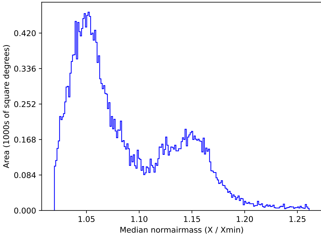
ddf_acor_sf15_ls20_lsr10_v3.4_10yrs All sky z band: Median normairmass
