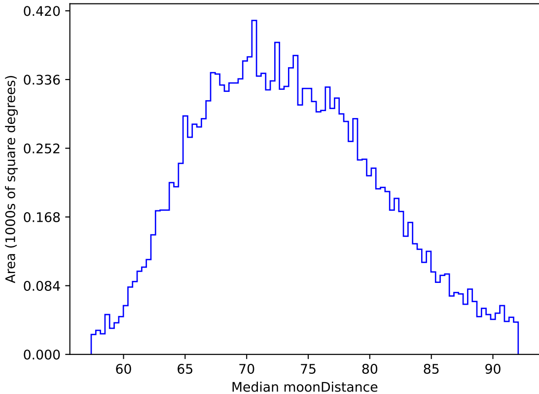
ddf_acor_sf15_lsf20_lsr10_v3.4_10yrs WFD z band: Median moonDistance
