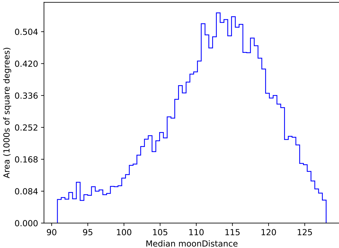
ddf_acor_sf15_lsf20_lsr10_v3.4_10yrs WFD r band: Median moonDistance
