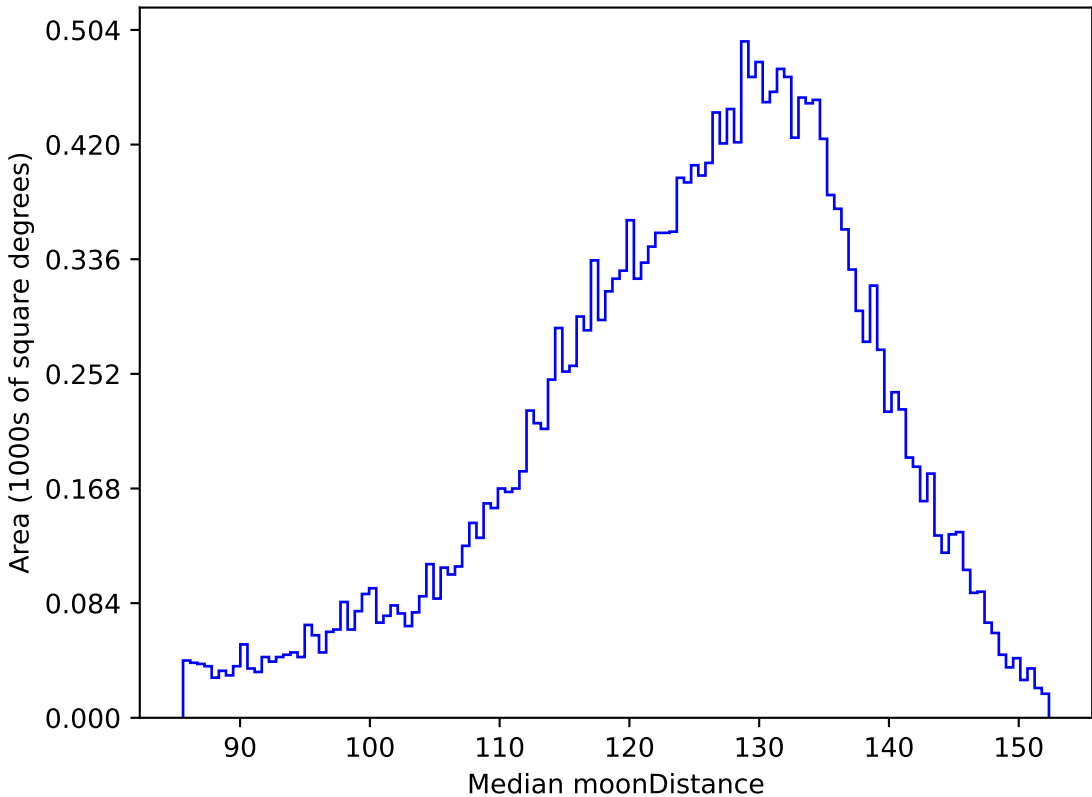
ddf_acor_sf15_lsf20_lsr10_v3.4_10yrs All sky u band: Median moonDistance
