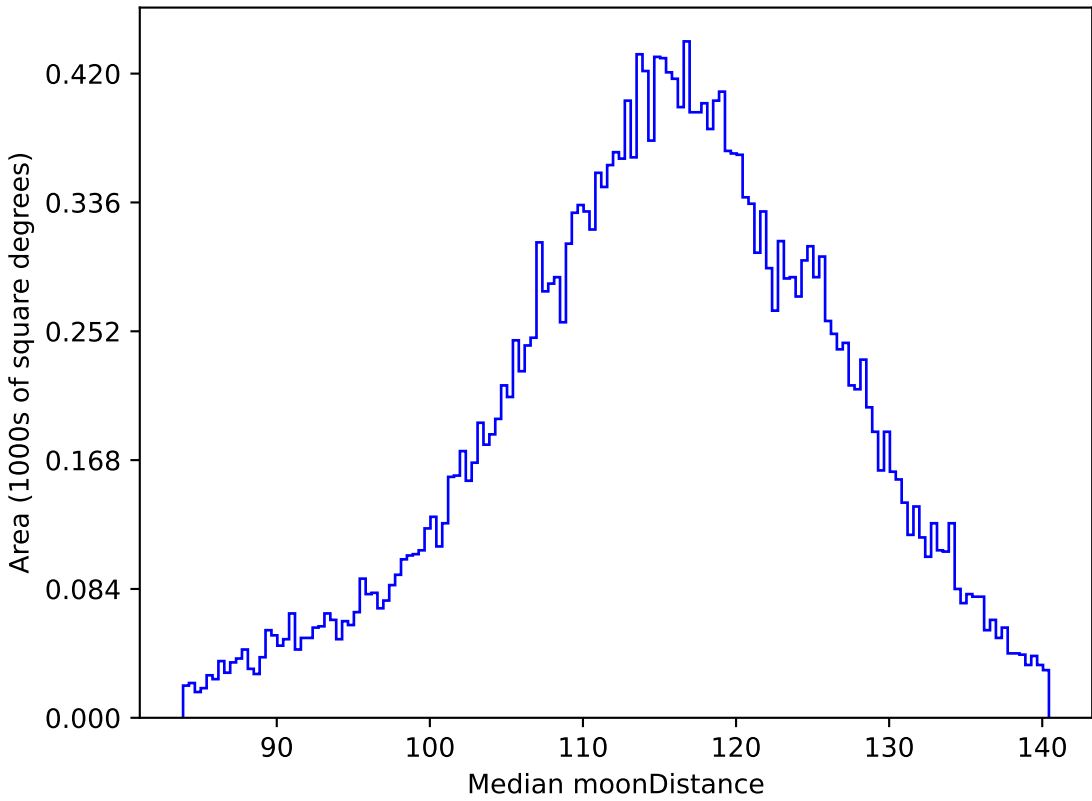
ddf_acor_sf15_lsf20_lsr10_v3.4_10yrs All sky g band: Median moonDistance
