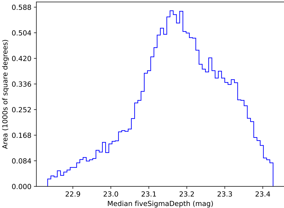
ddf_acor_sf15_lsf20_lsr10_v3.4_10yrs WFD u band: Median fiveSigmaDepth
