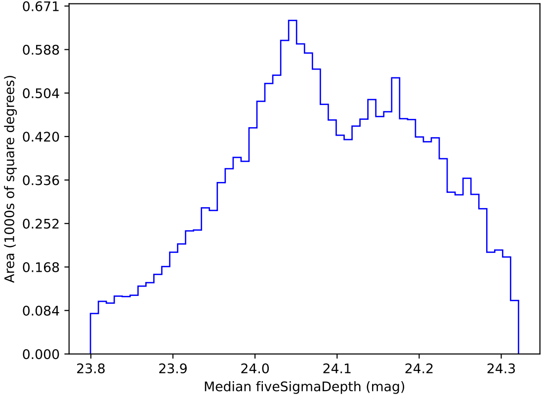
ddf_acor_sf15_lsf20_lsr10_v3.4_10yrs WFD r band: Median fiveSigmaDepth
