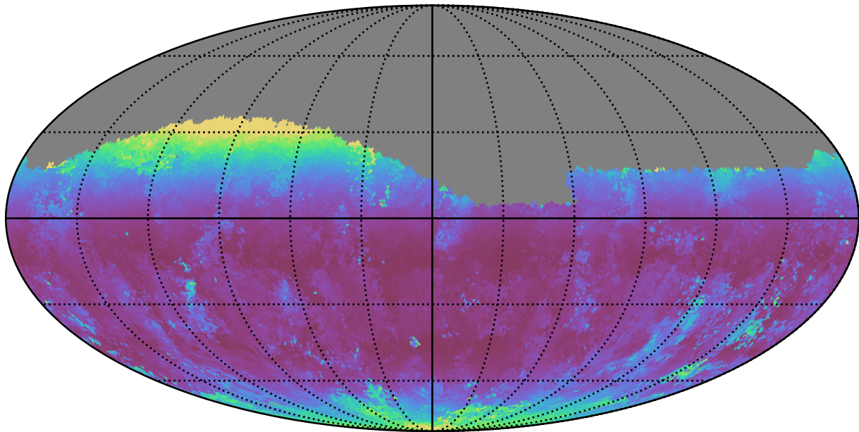
ddf_acor_sf15_lsf20_lsr10_v3.4_10yrs Yr 1 g band: Median airmass
