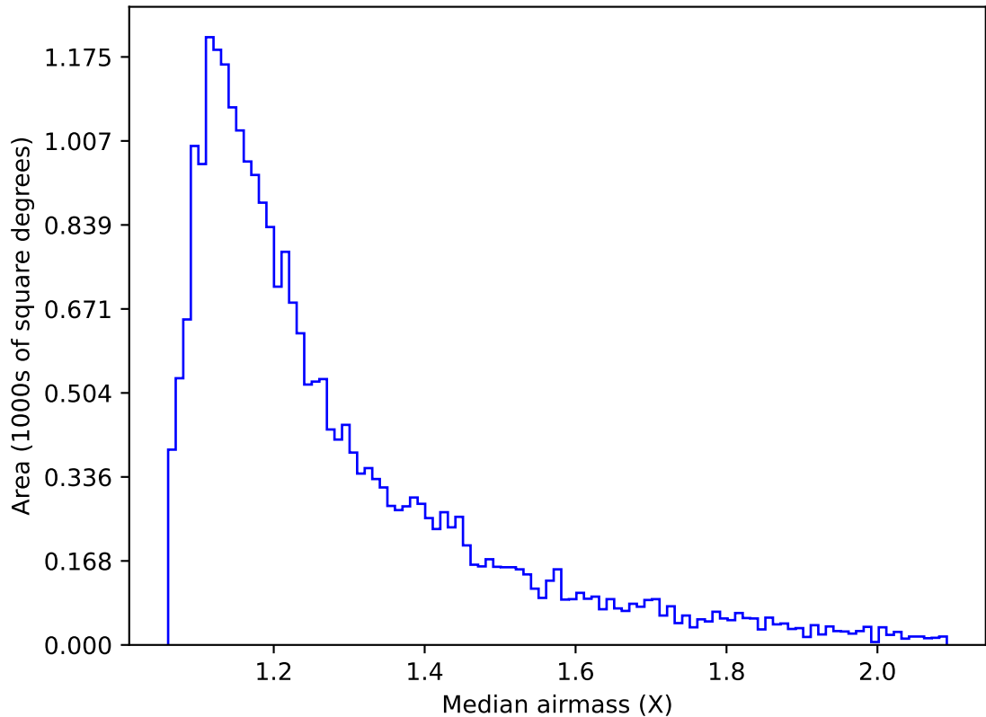
ddf_acor_sf15_lsf20_lsr10_v3.4_10yrs Yr 1 g band: Median airmass
