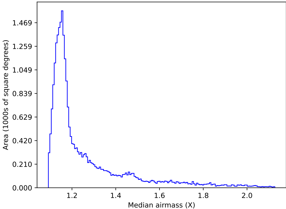
ddf_acor_sf15_lsf20_lsr10_v3.4_10yrs All sky z band: Median airmass
