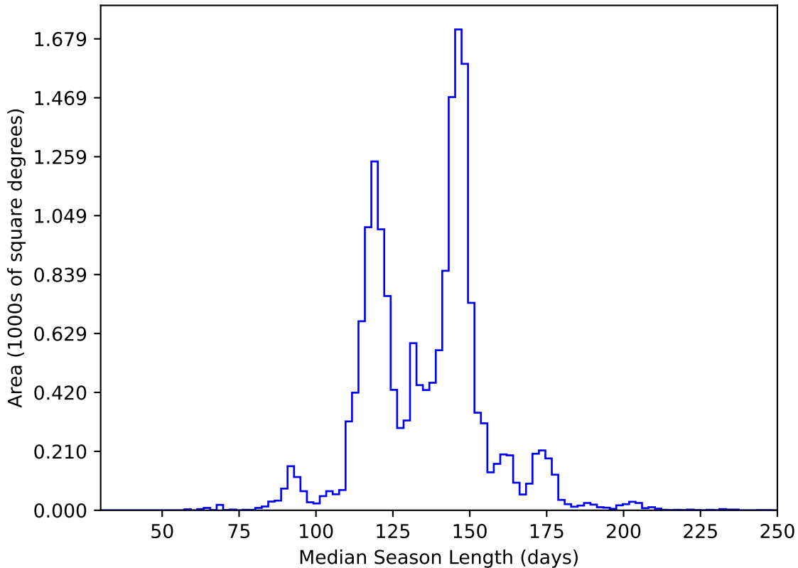
ddf_acor_sf15_lsf20_lsr10_v3.4_10yrs WFD y band: Median Season Length
