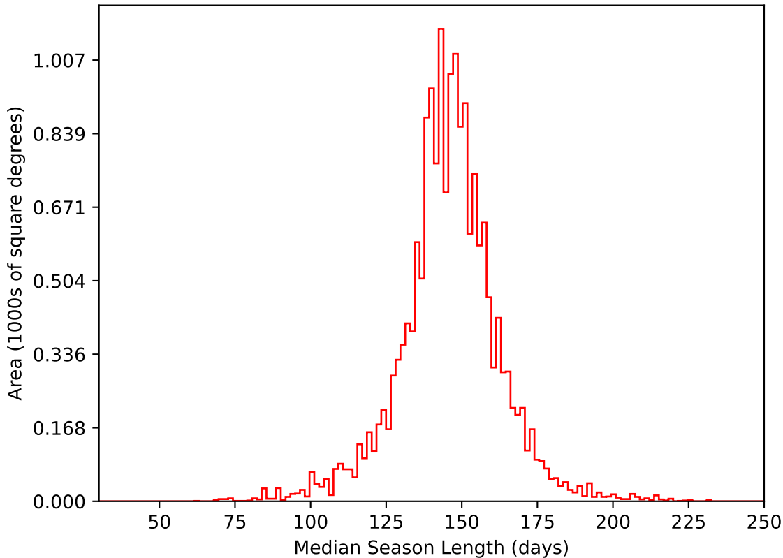
ddf_acor_sf15_lsf20_lsr10_v3.4_10yrs WFD i band: Median Season Length
