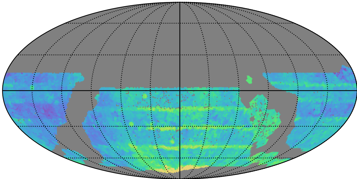
ddf_acor_sf15_lsf20_lsr10_v3.4_10yrs WFD all bands: Median Season Length
