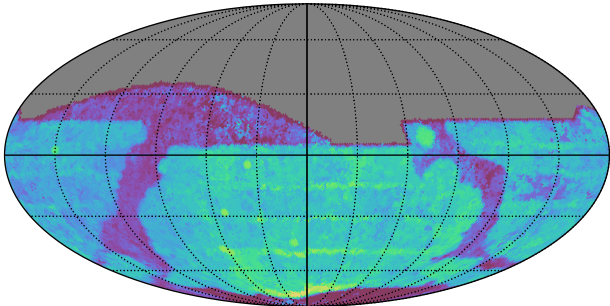
ddf_acor_sf15_lsf20_lsr10_v3.4_10yrs All sky z band: Median Season Length
