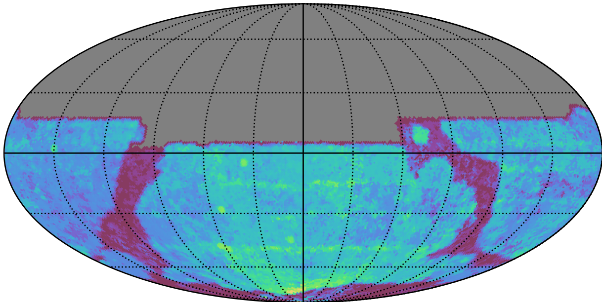
ddf_acor_sf15_lsf20_lsr10_v3.4_10yrs All sky y band: Median Season Length
