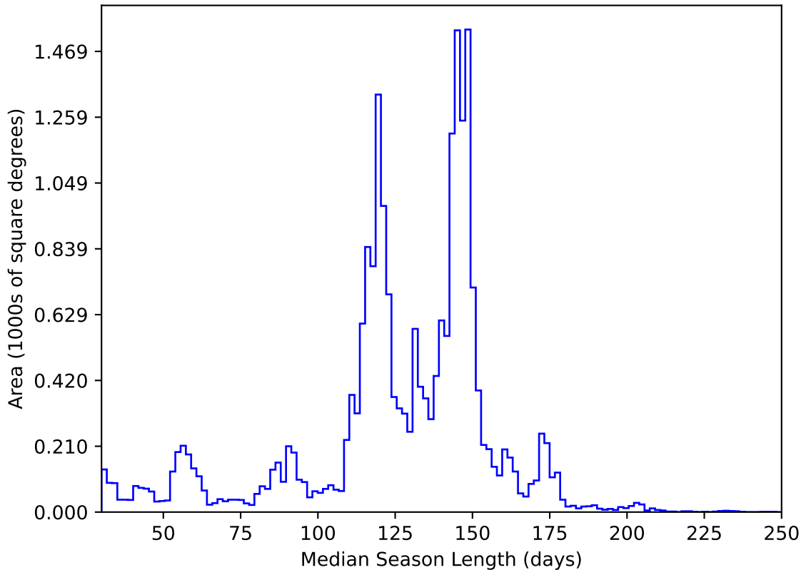
ddf_acor_sf15_lsf20_lsr10_v3.4_10yrs All sky y band: Median Season Length
