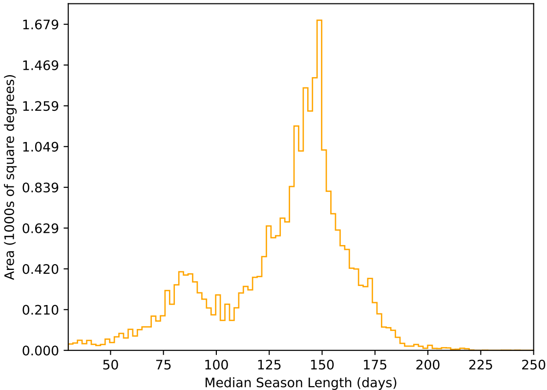
ddf_acor_sf15_lsf20_lsr10_v3.4_10yrs All sky r band: Median Season Length
