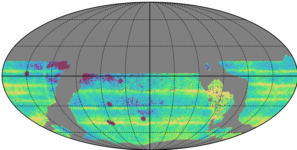
ddf_acor_sf15_lsf20_lsr10_v3.4_10yrs WFD: Median Intra-Night Gap
