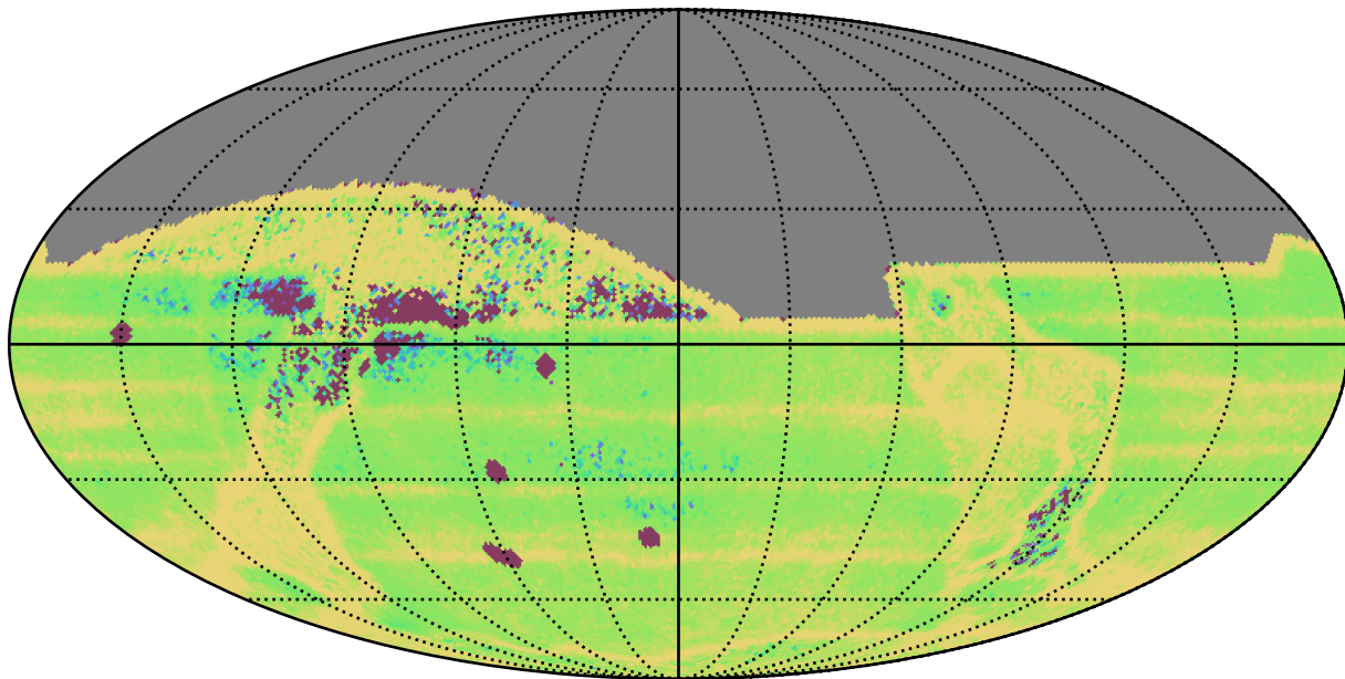
ddf_acor_sf15_lsf20_lsr10_v3.4_10yrs All sky: Median Intra-Night Gap
