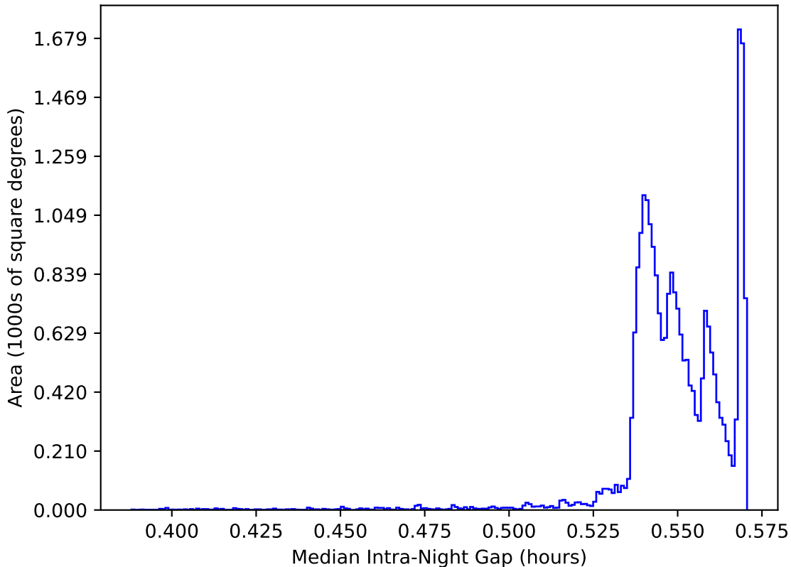
ddf_acor_sf15_lsf20_lsr10_v3.4_10yrs All sky: Median Intra-Night Gap
